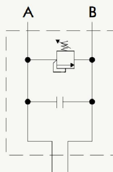
ANTI-SHOCK VALVE WITH CROSS RETURN ON PORT A 溢流閥，控制工作口A
