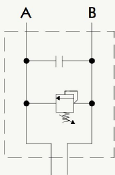
ANTI-SHOCK VALVE WITH CROSS RETURN ON PORT B 溢流閥，控制工作口B
